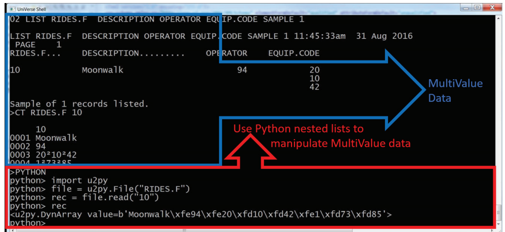
Figure 1: Working with Python from within UniData
